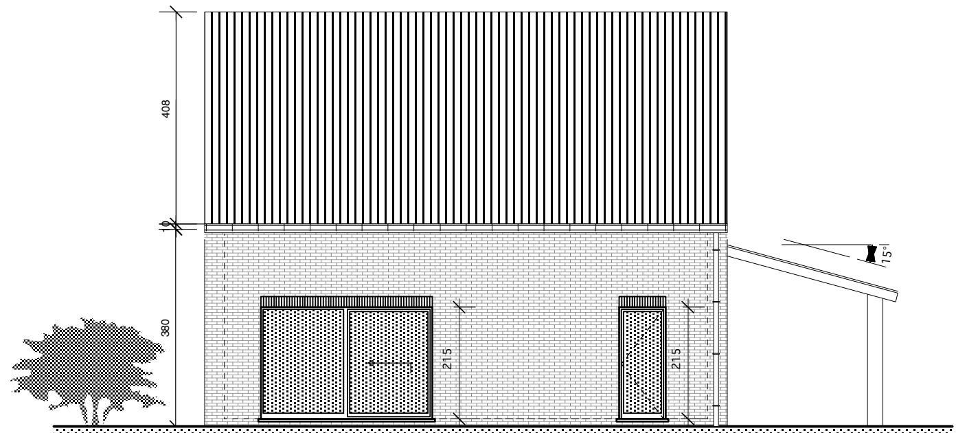
FACADE ARRIERE
